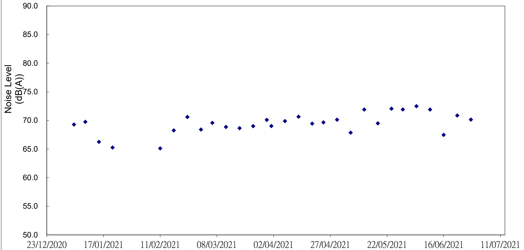
Noise Level (Leq 30 mins) dB(A) Vs Date for Location W-N18
